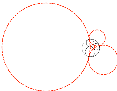
Figure 3. Dual circles
