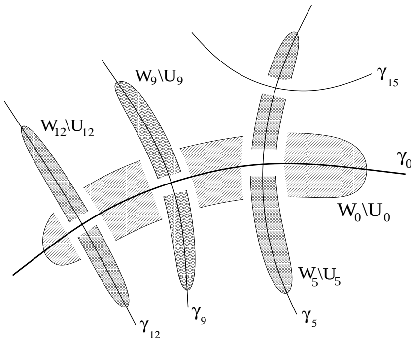
Figure 1. Avoiding self-intersections.
